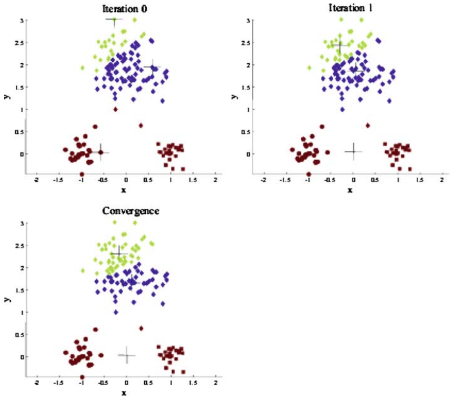
Fig. 2 Effect of an inferior initialization on the k -means results
